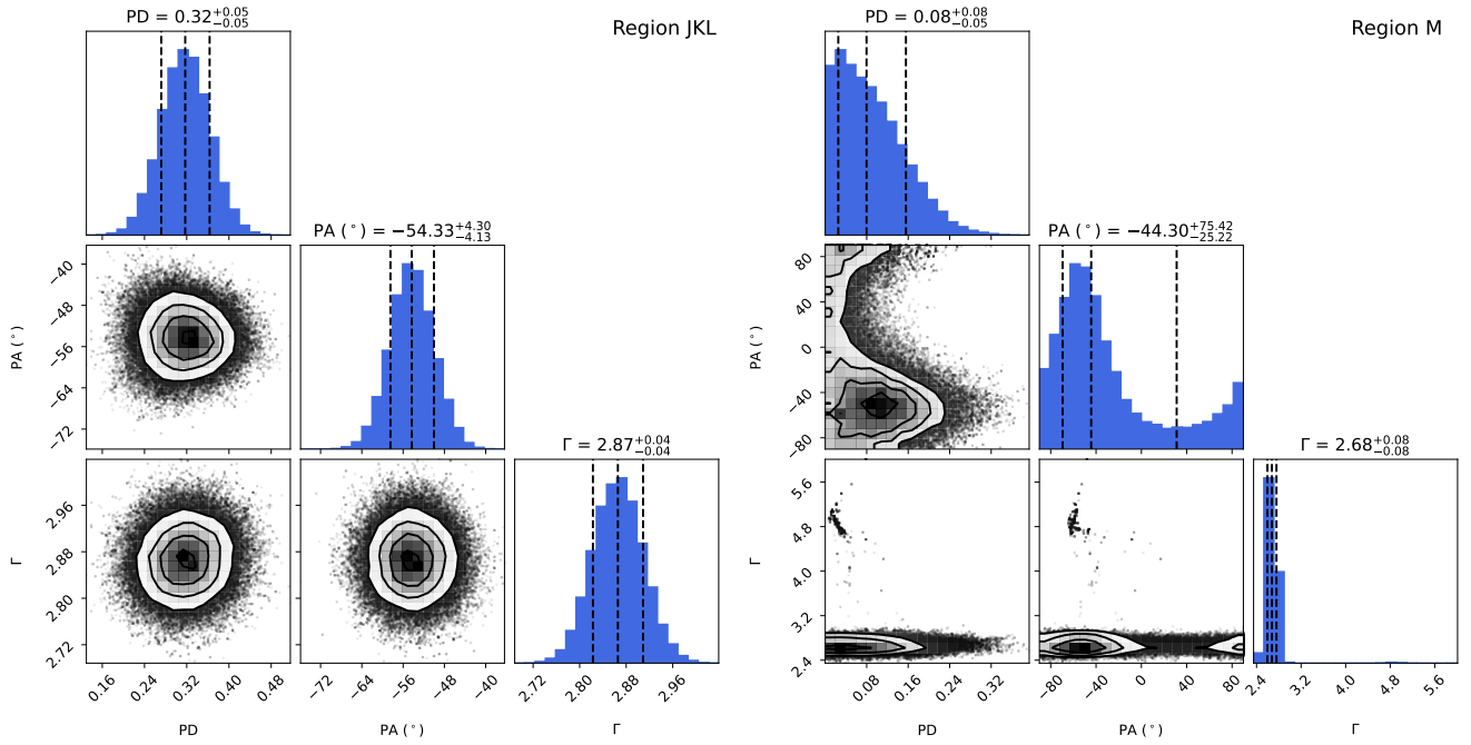
Figure 9. Two-dimensional correlation distributions of parameters in the spectro-polarimetric analysis for regions JKL (left) and M (right). The contours provide the 0.5, 1, 1.5, 2 \sigma equivalent range. The histograms show the posterior distribution of PD, PA, and spectral index \Gamma , and the vertical lines denote the 0.16, 0.5, and 0.84 quantiles of the samples.
